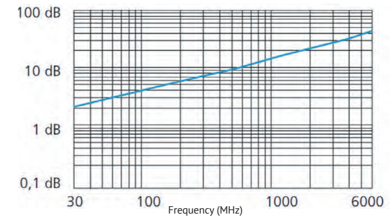
Typ. Attenuation (dB/100 m at 20 °C)
