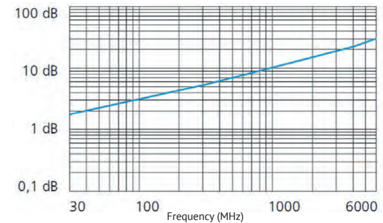
Typ. Attenuation (dB/100 m at 20 °C)
